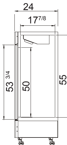
Side View MCF8725
